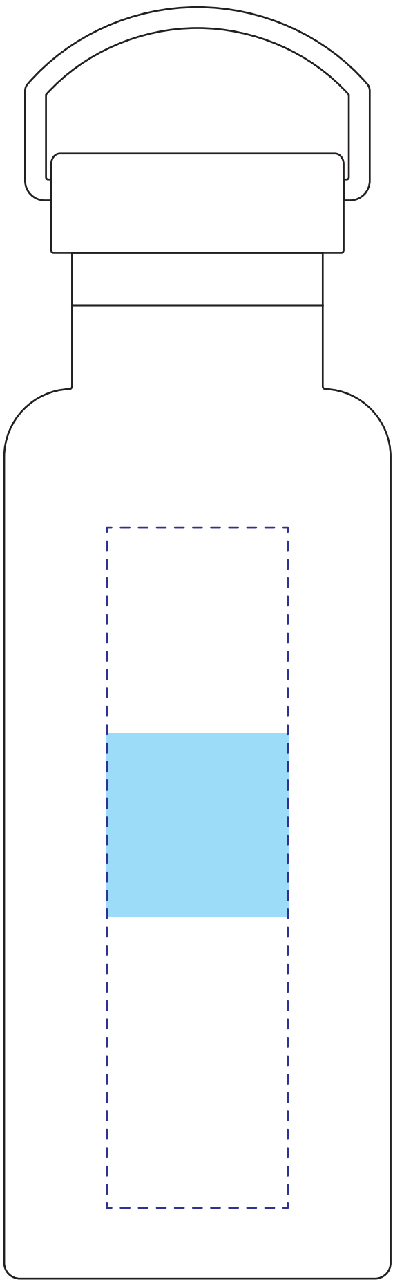
側面：W35×H35mm
